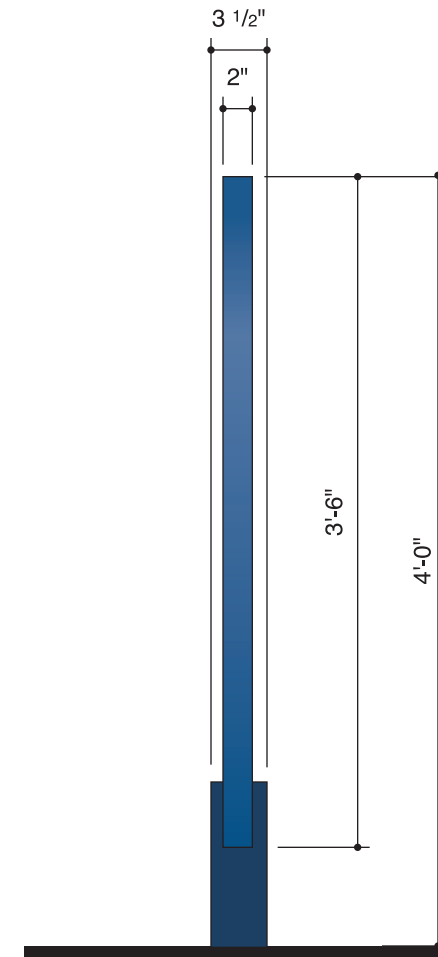
2 Elevation - Sides C/D scale: 1"=1'-0"
